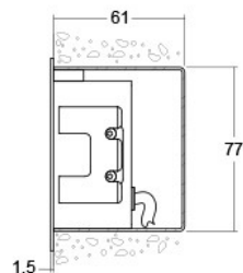
Side section view
