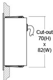
Side section view
