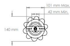
Ceiling Rose Detail
